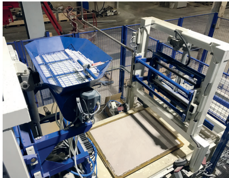
Plastic ball introduction into fresh products
